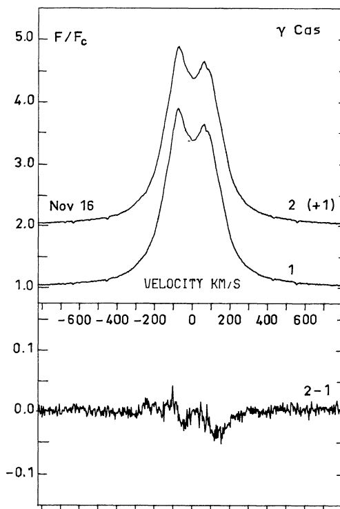
Fig. 6. Same as in Fig. 5. Spectra were obtained in 1981 Nov. 16, UT's are as follows: 1: 6 h 03 m ; 2: 8 h 22 m
