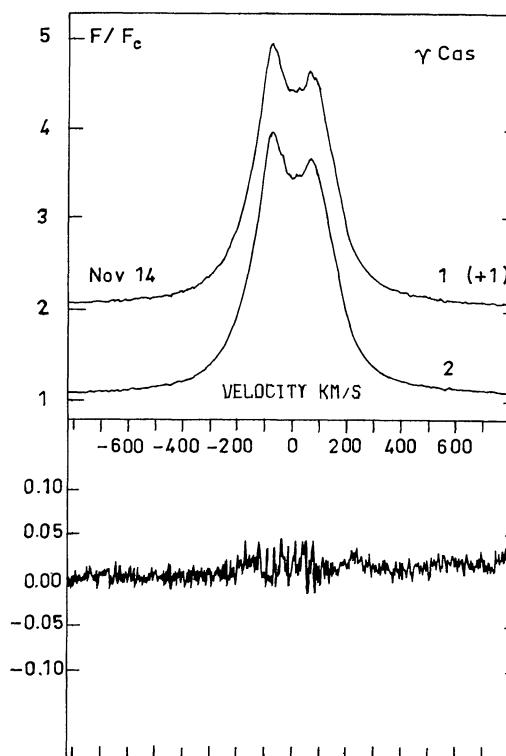
Fig. 5. Variations of the H_\alpha line profile of \gamma Cas during one night. Spectra were obtained in 1981 Nov. 14, UT's are as follows: 1: 6 h 08 m ; 2: 10 h 55 m . Value of a constant added to the spectrum plot is indicated in brackets
