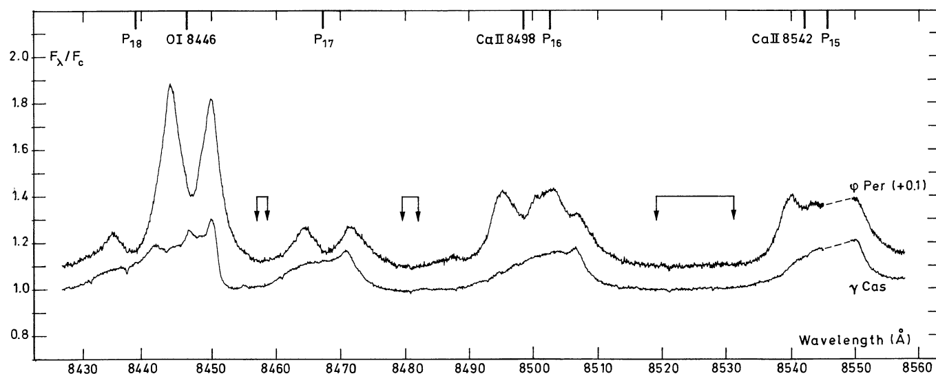
Fig. 2. Typical spectra obtained in the \lambda 8500 \text{ \AA} region. Arrows indicate the location of bands used for the continuum level determination. The spectra were obtained in 1981 Nov. 16
