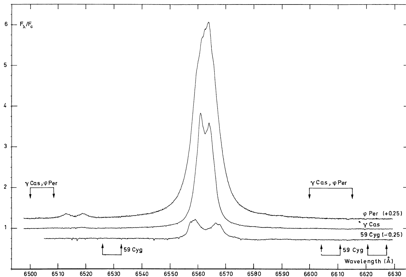
Fig. 1. Typical spectra obtained in the H_x region. Arrows indicate the location of bands used for the continuum level determination. The value of a constant added to the plot is indicated in brackets just after the star name. The presented spectra of \gamma Cas and \phi Per were obtained in 1981 Nov. 15, that of 59 Cyg in 1982 June 6
